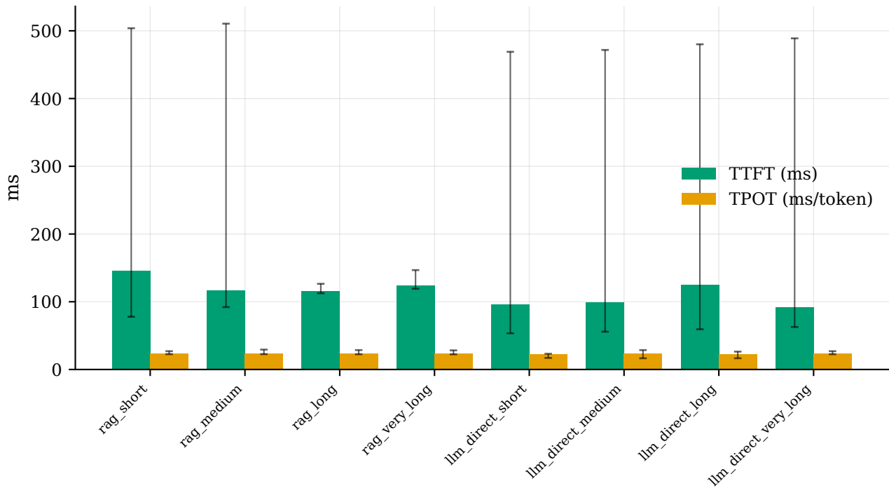
Streaming latency (tok64) — mean, min-max
