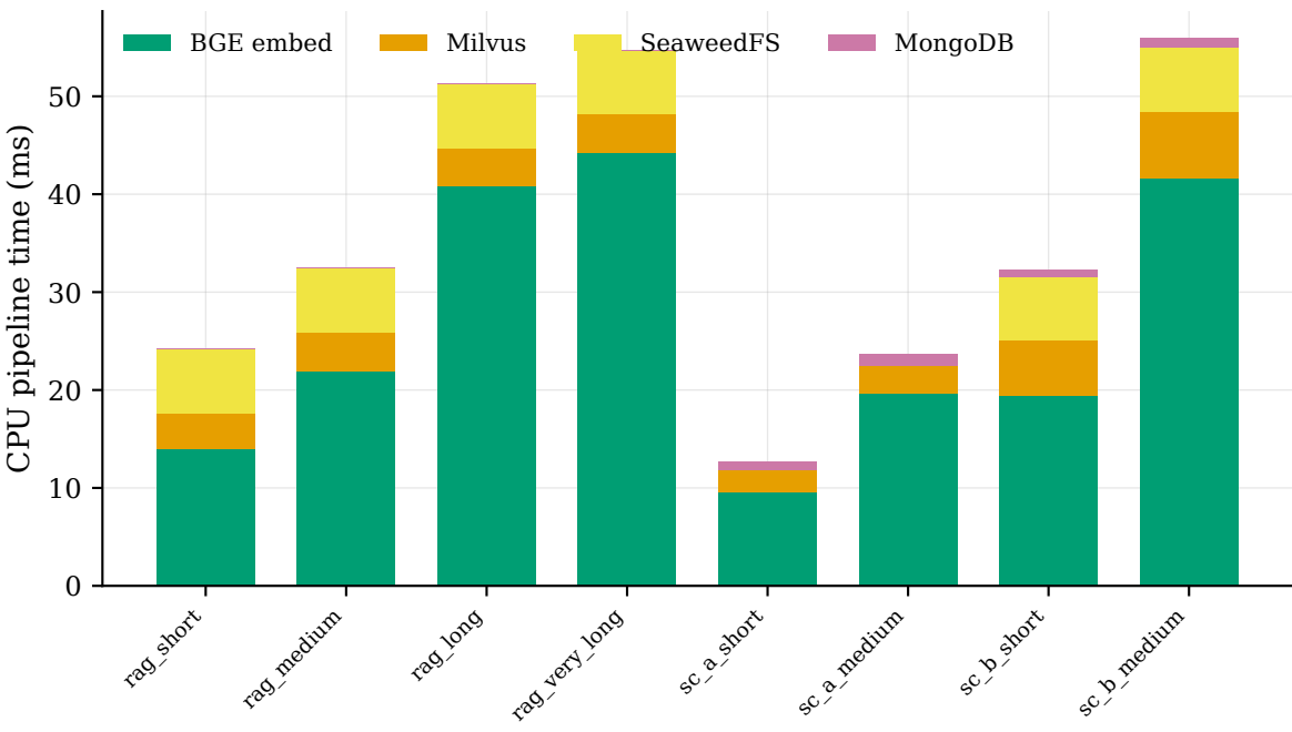
Frontend pipeline cost per cell (tok320) — GPU excluded
