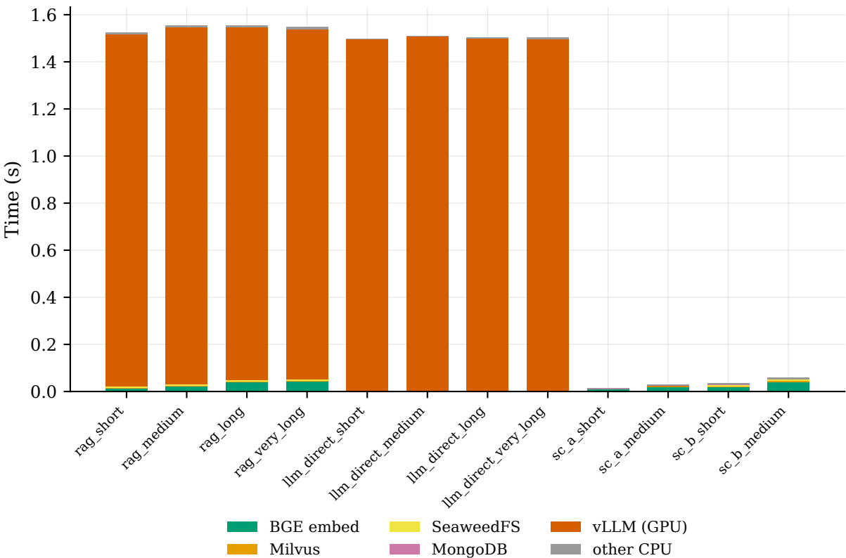
Request time decomposition (tok64)
