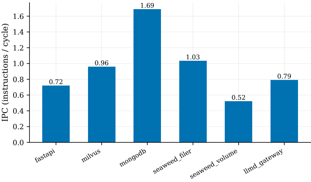
Per-pod IPC (rag_medium, tok64)
