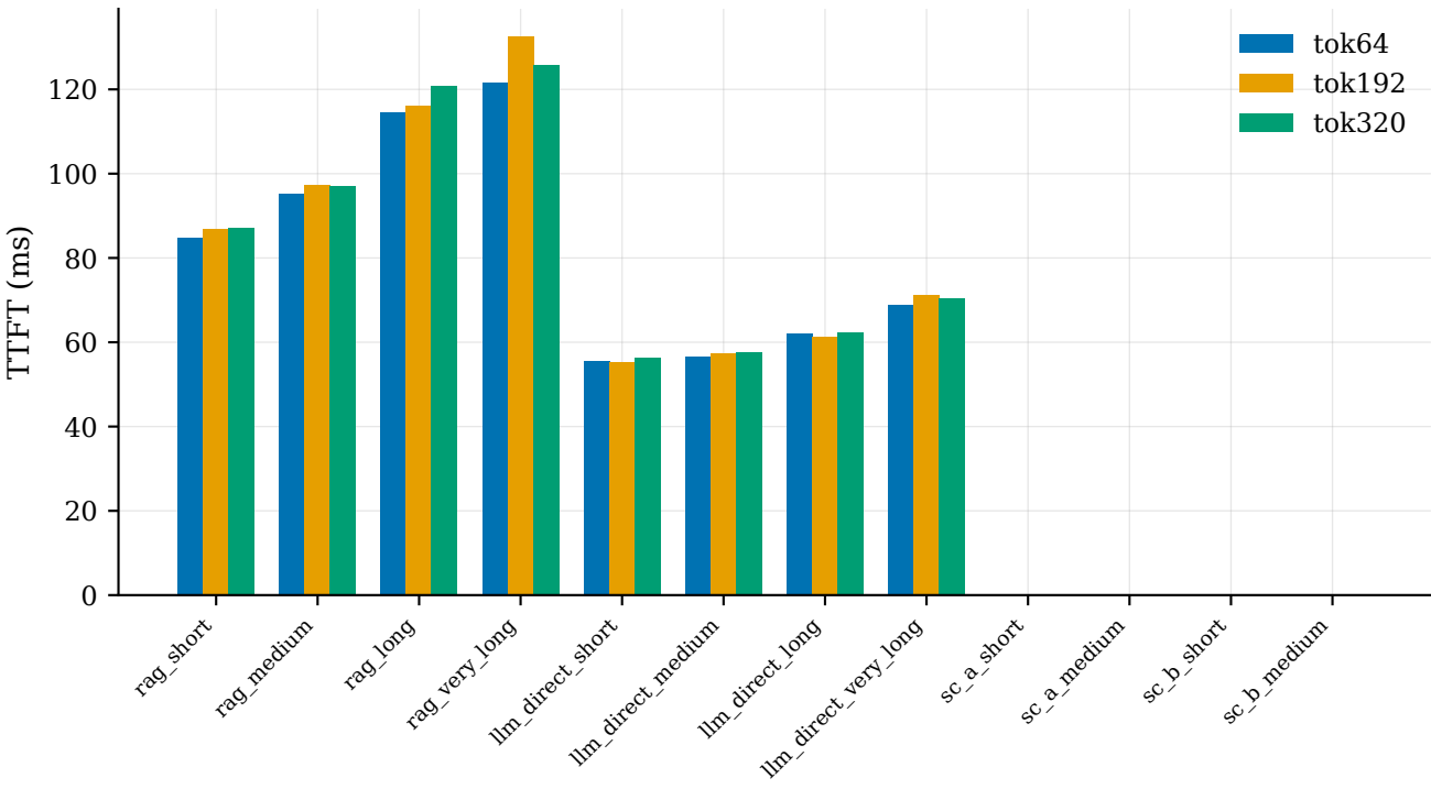
TTFT per cell across tiers
