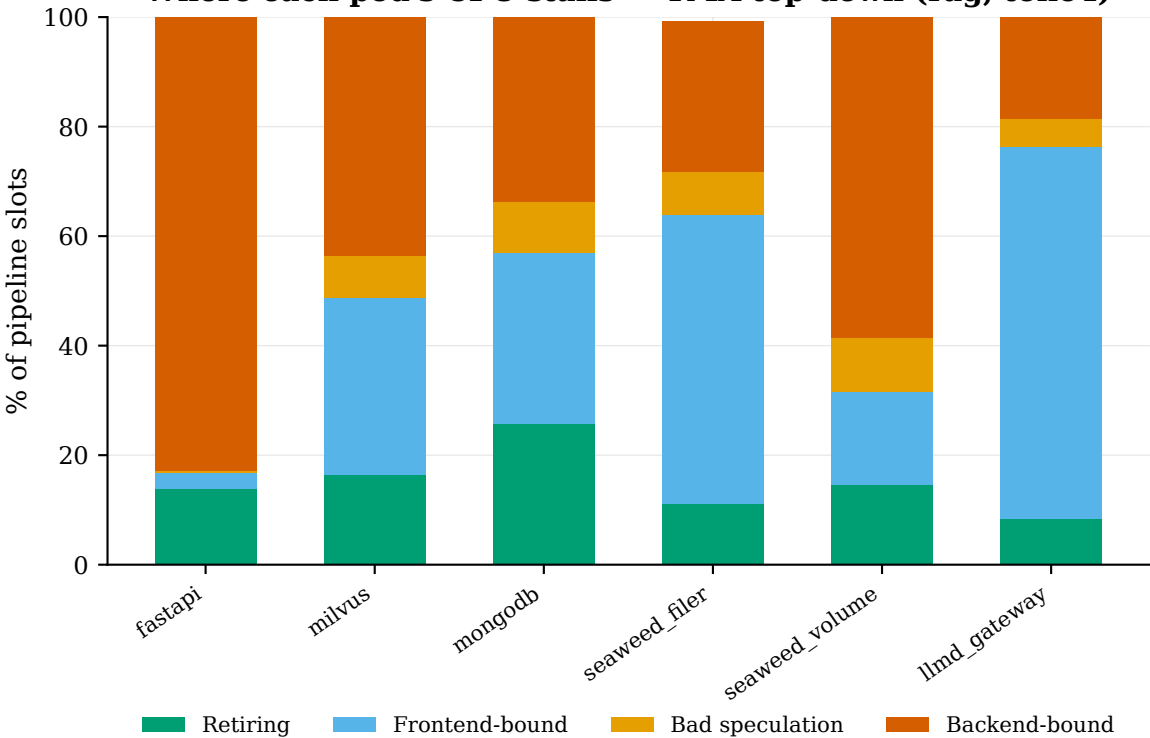
Where each pod's CPU stalls — TMA top-down (rag, tok64)
