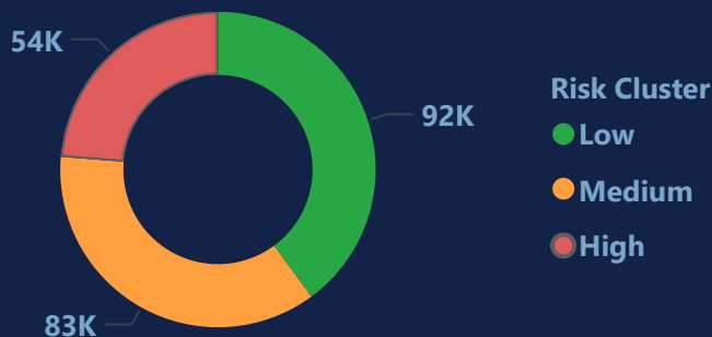
Population Distribution by Cluster
