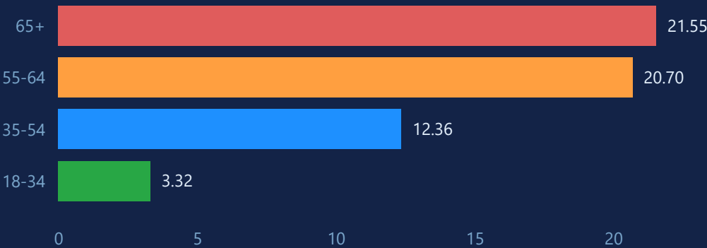
Diabetes Rate by Age Group
