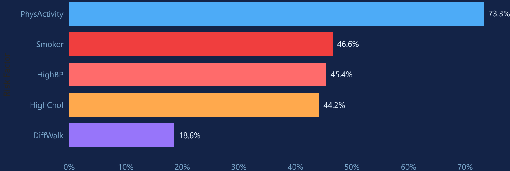
Population Risk Factors
