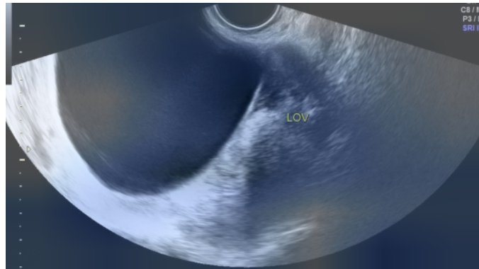
Classification Grad-CAM
