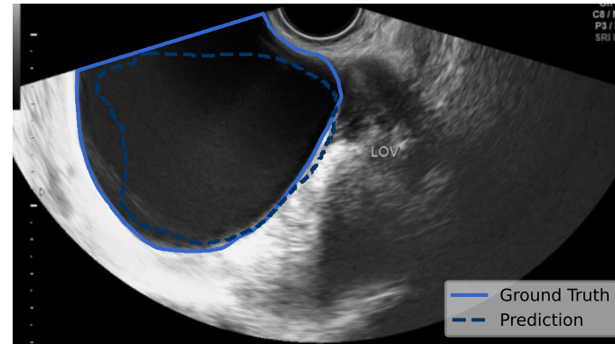
Segmentation Prediction
