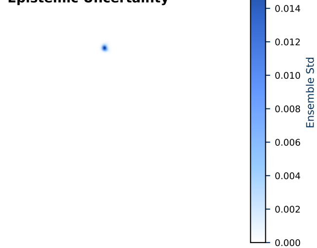
Epistemic Uncertainty
