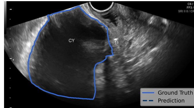
Segmentation Prediction
