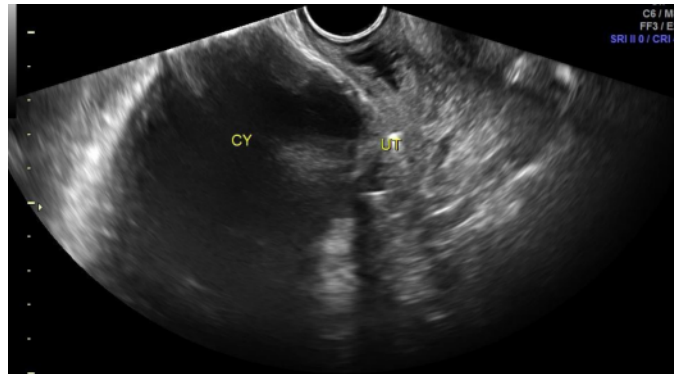
Original Ultrasound
