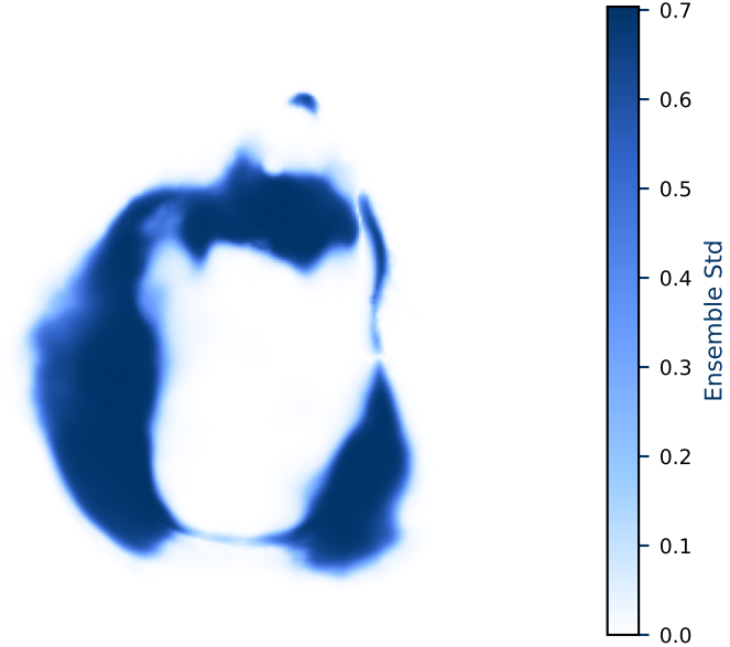
Epistemic Uncertainty
