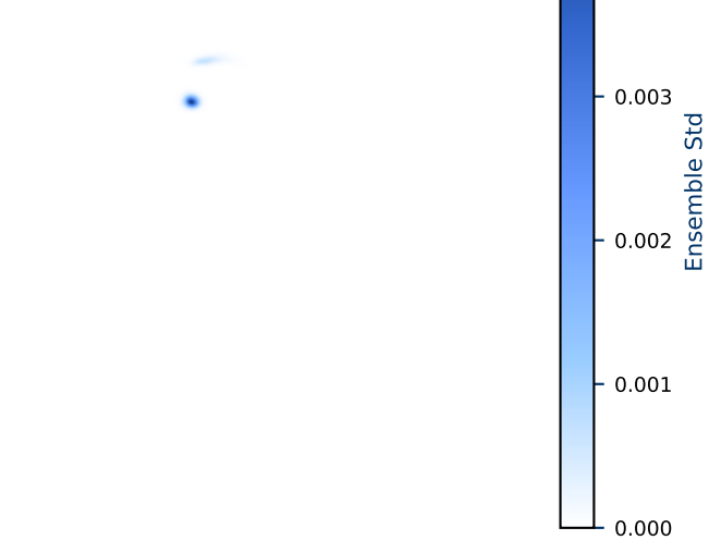
Epistemic Uncertainty
