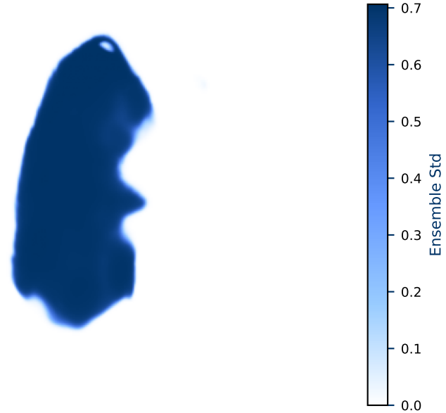
Epistemic Uncertainty
