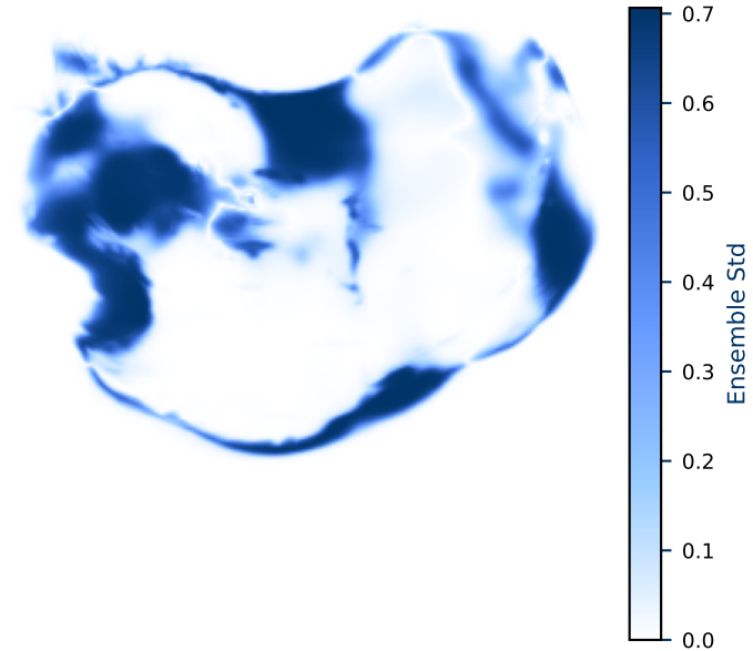
Epistemic Uncertainty
