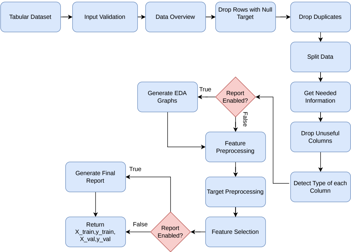
Figure 4.6: Tabular Preprocessing Workflow
