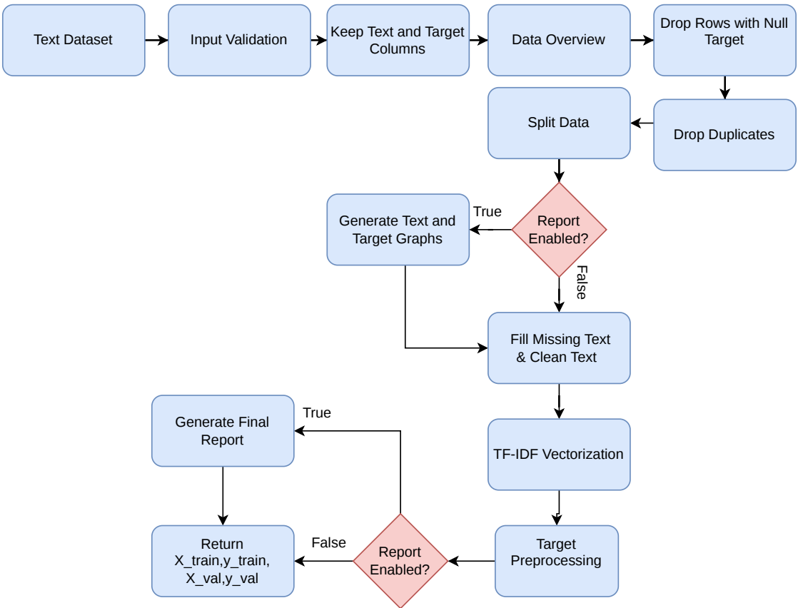
Figure 4.7: Text Preprocessing Workflow
