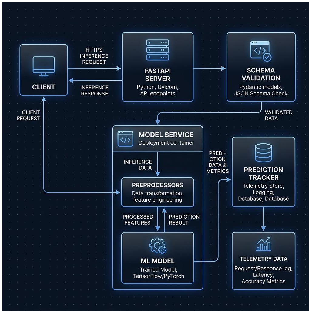
Figure 4.5: Model Serving Architecture and Execution Flow
