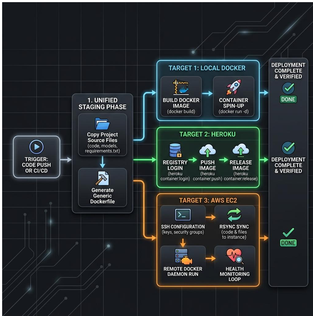
Figure 4.6: Multi-Target Deployment Orchestration Flow
