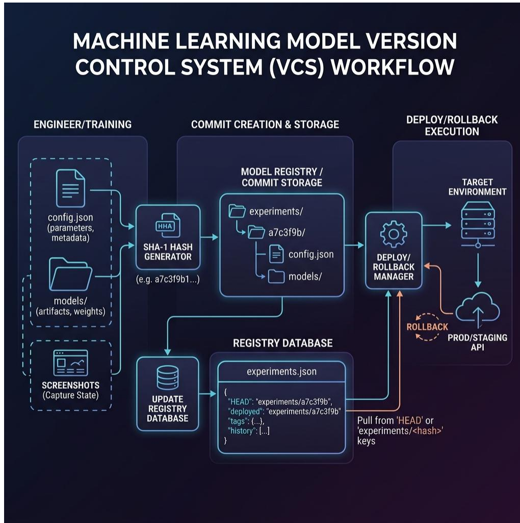
Figure 4.7: Model Version Control System (VCS) Workflow
