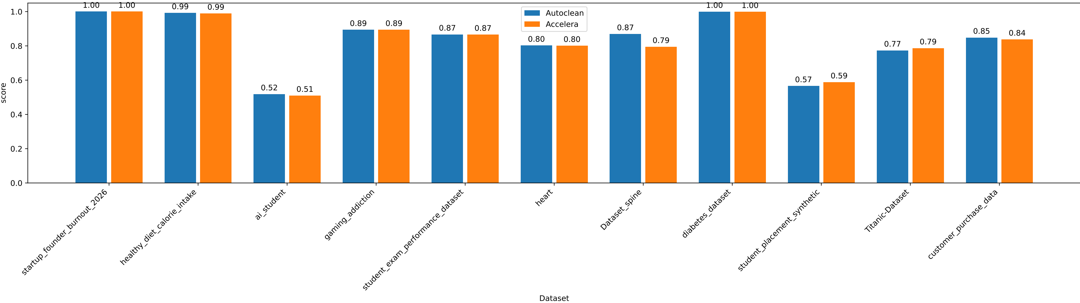
classification - AutoClean vs Accelera LR
