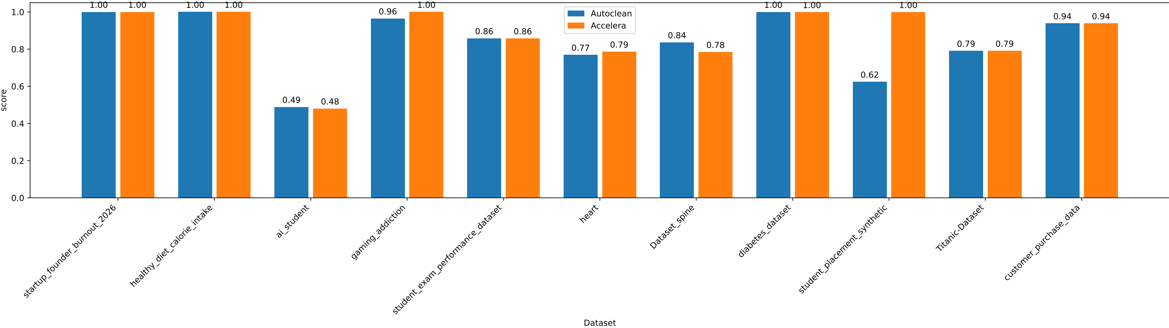
classification - AutoClean vs Accelera RandomForest
