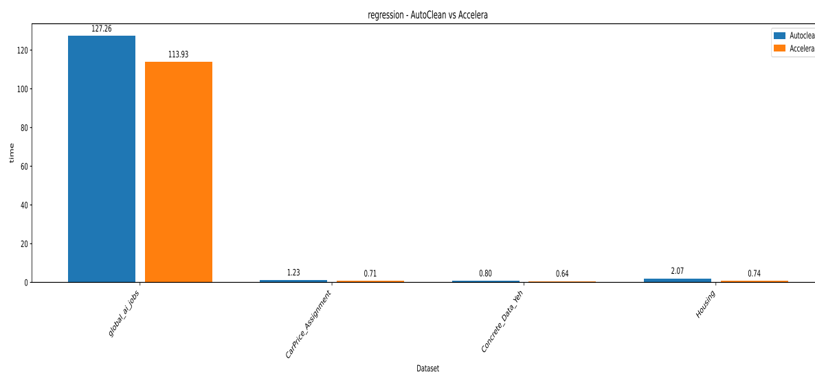
Figure 5.4: Regression Preprocessing Time Comparison
