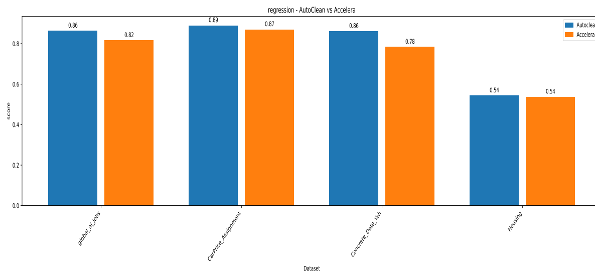
Figure 5.3: Regression Performance Comparison ( R^2 Score)
