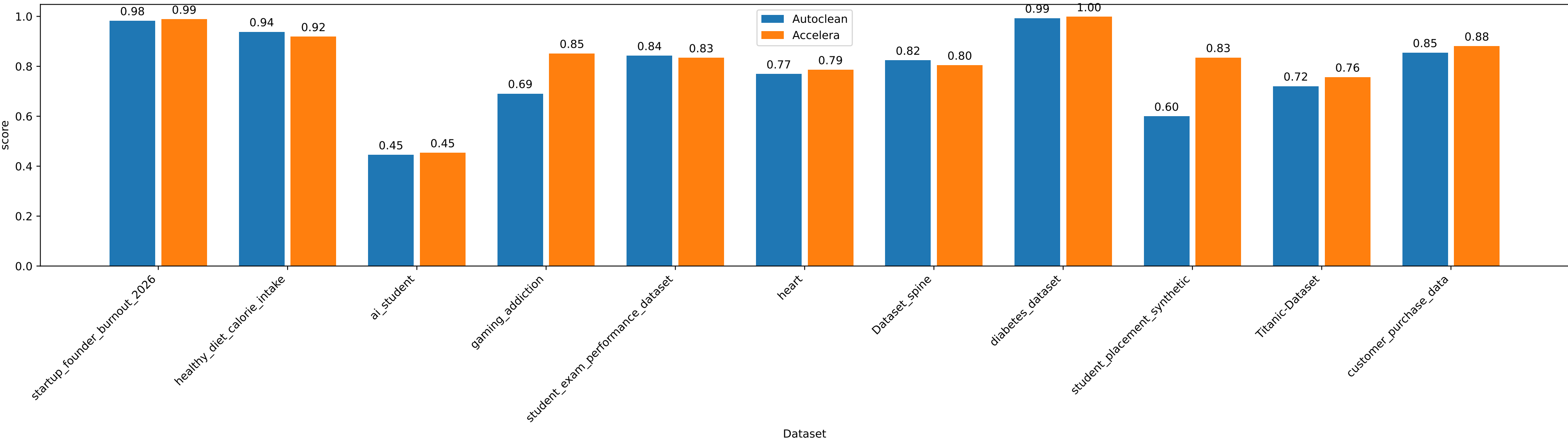
classification - AutoClean vs Accelera KNN
