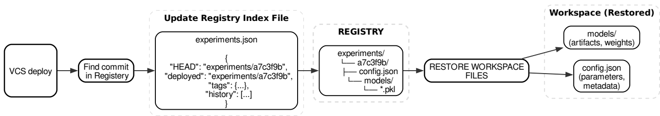
Figure 4.13: VCS Deploy Workflow
