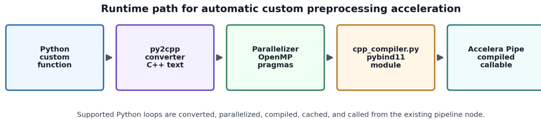
Figure 4: Architecture of the integration between custom Python preprocessing, the Python-to-C++ converter, the OpenMP parallelizer, the native compiler, and accelera_pipe .
