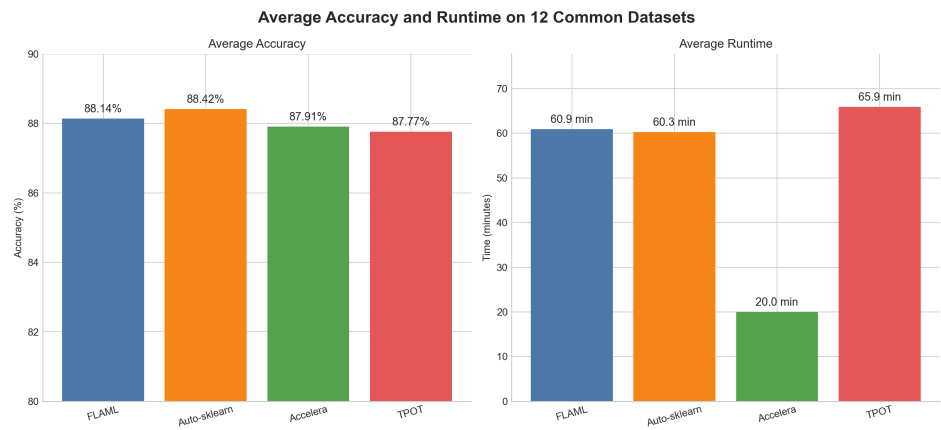
Figure 5.1: Mean classification accuracy and runtime for the evaluated AutoML systems.
