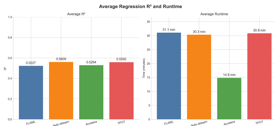
Figure 5.4: Mean regression R^2 and runtime for the evaluated AutoML systems.
