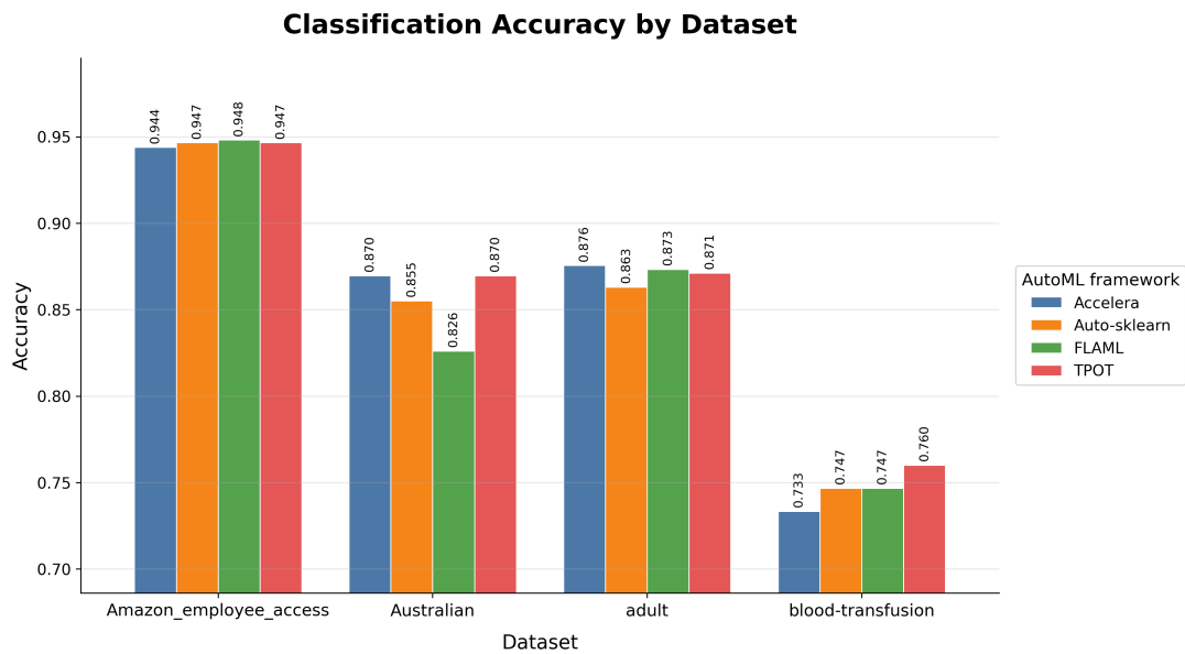
Figure 5.2: Per-dataset classification accuracy on common datasets.
