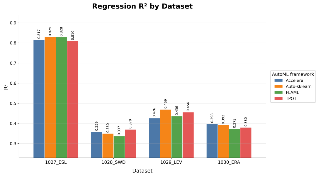
Figure 5.5: Per-dataset regression R^2 on common datasets.
