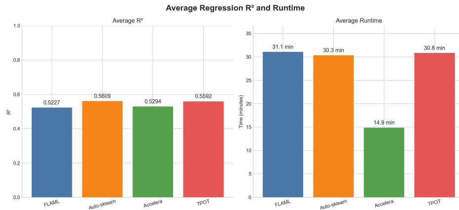
Figure 5.2: Mean regression R^2 and runtime for the evaluated AutoML systems
