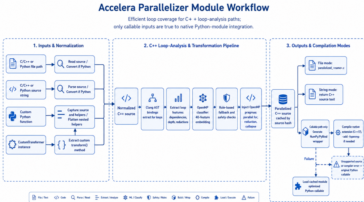
Figure 4.4: Code Parallelizer module workflow
