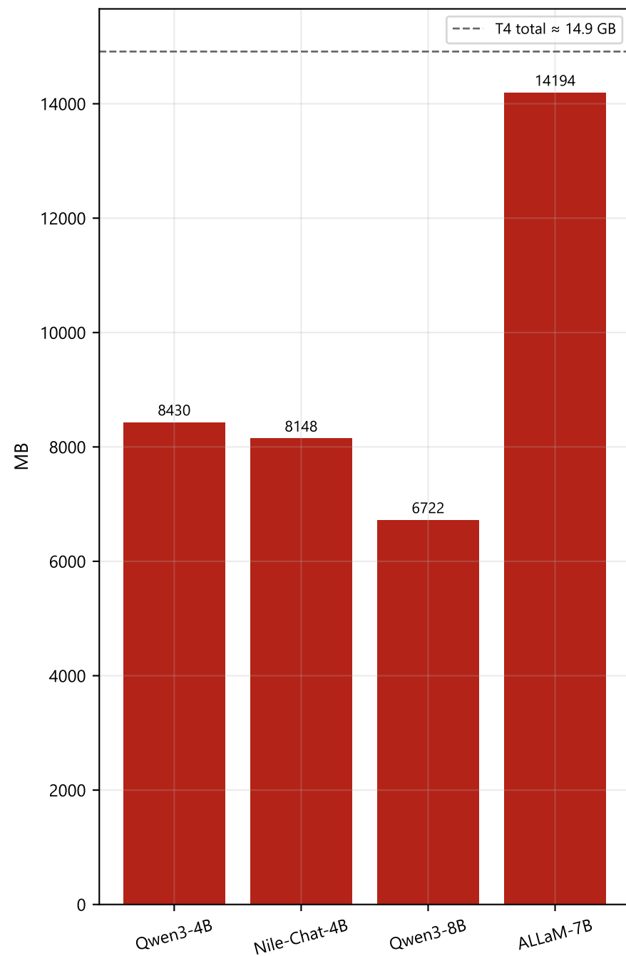
Peak VRAM on Tesla T4
