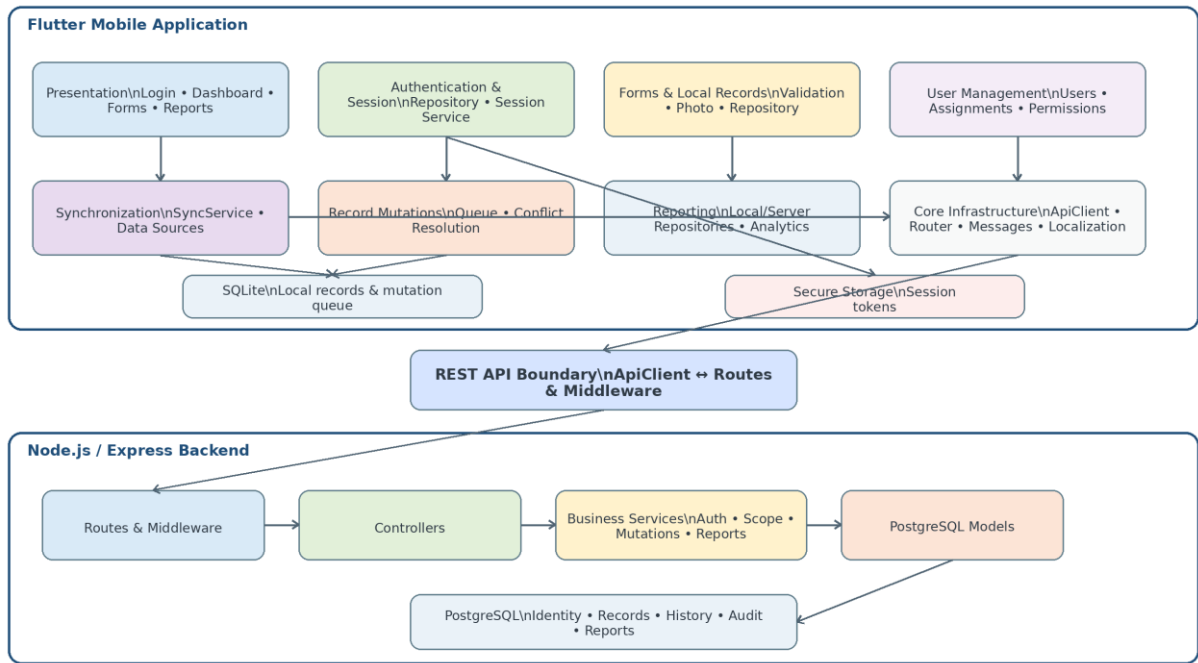
Figure 8. SyncField component diagram.
