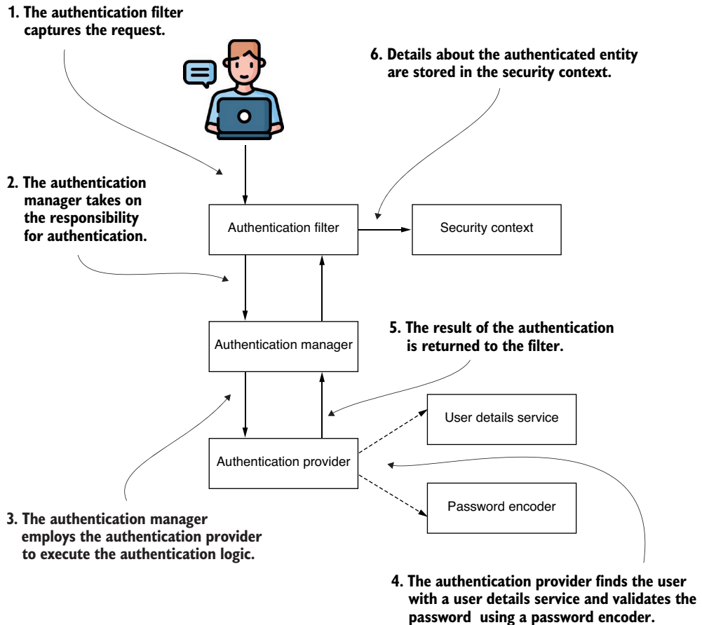
Figure 2.2 The core elements involved in Spring Security's authentication process and their interconnections are the focus here. This framework forms the essential structure for executing authentication using Spring Security. Throughout the book, we will frequently reference this architecture while examining various authentication and authorization strategies.
