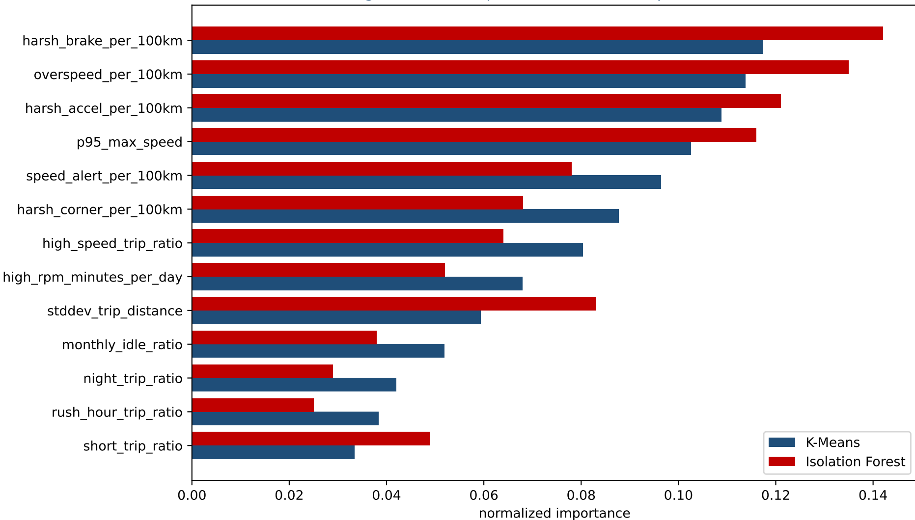
Surrogate feature importance for the unsupervised models
