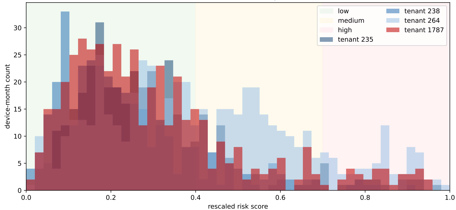
Distribution of the risk score per tenant
