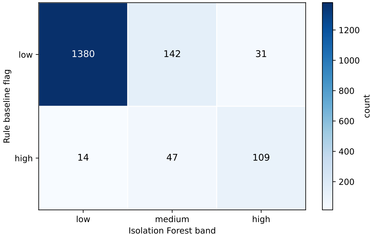
Confusion matrix: rule vs Isolation Forest
