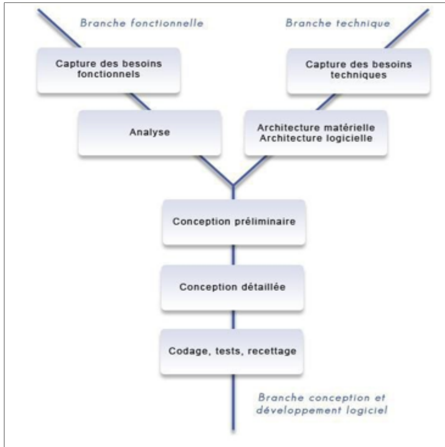
Figure 1.6: Processus en Y.
