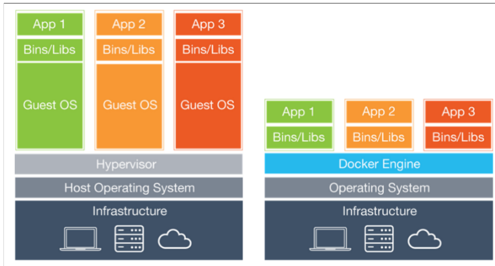
Figure 2.1: Machine virtuelle vs docker.
