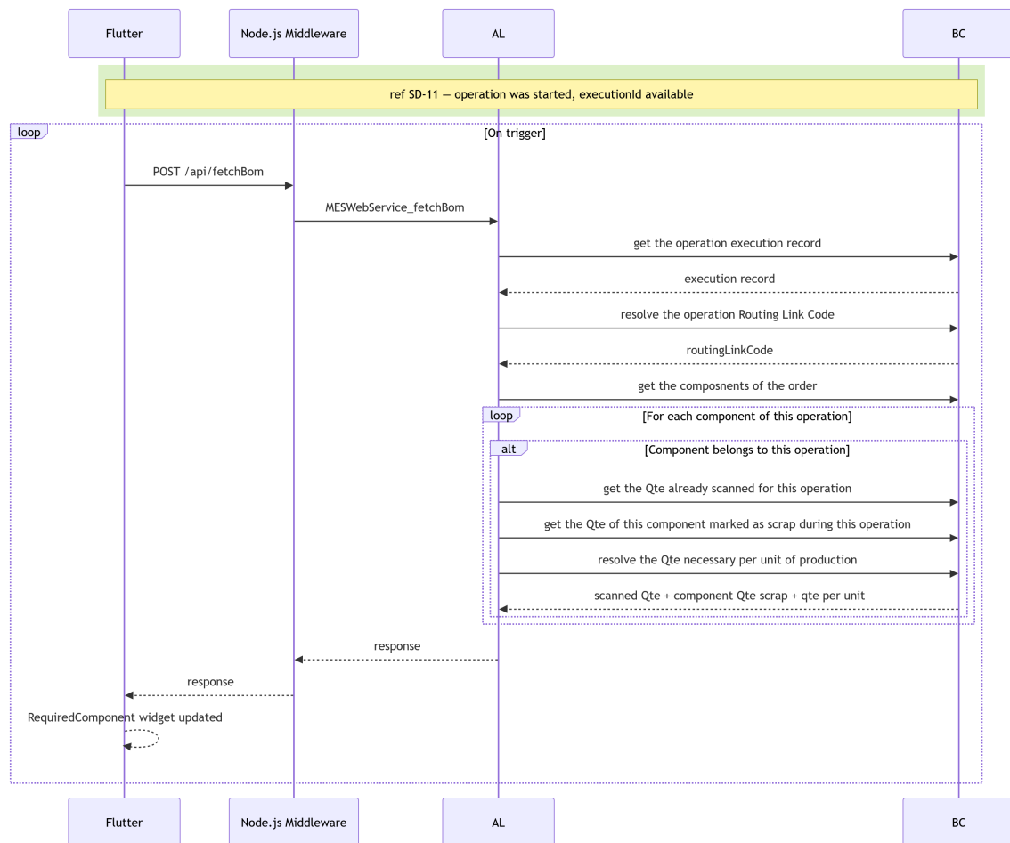
Figure 5.3. SD-21: Fetch Bill of Materials.
