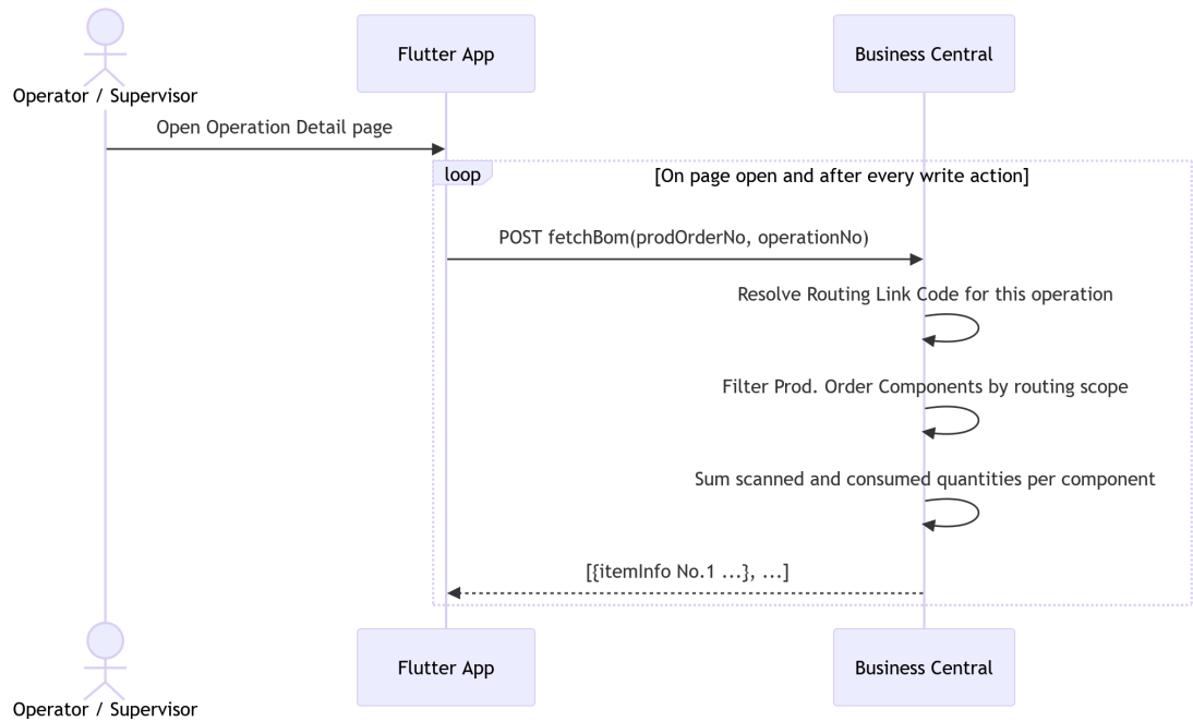
Figure 5.3. Sequence Diagram — Fetch Bill of Materials.
