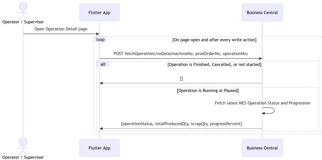
Figure 5.5. Sequence Diagram — Fetch Operation Live Data.
