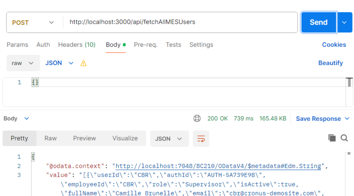
Figure 3.24. Postman endpoint test — fetchAllMesUsers .
