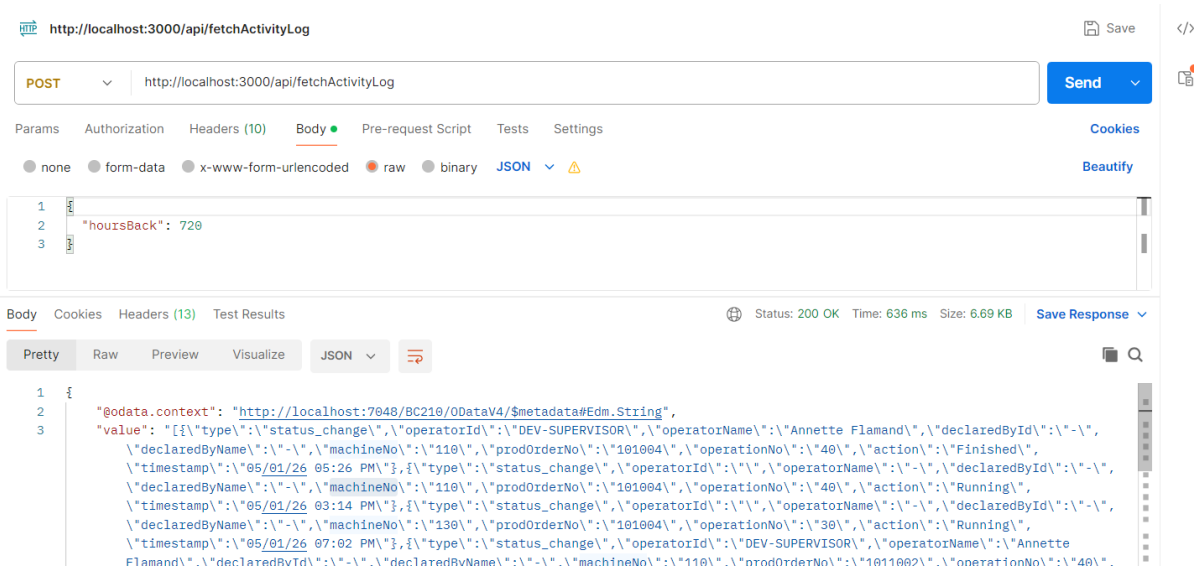
Figure 6.8. Postman endpoint test — fetchActivityLog .
