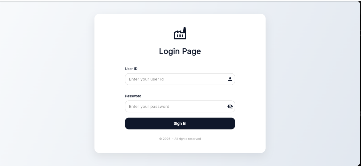
Figure 3.13. Login Page.
