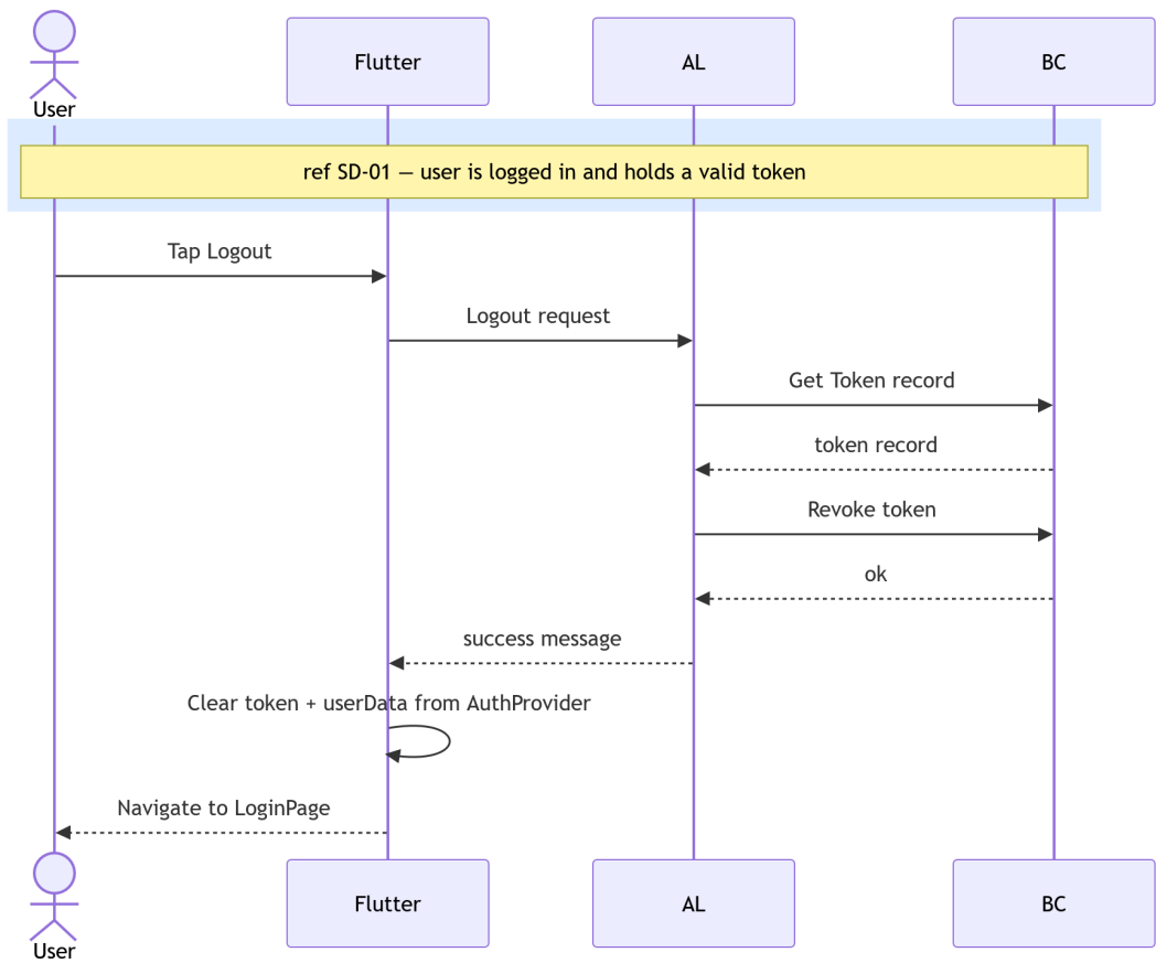
Figure 3.4. SD-03: Logout
