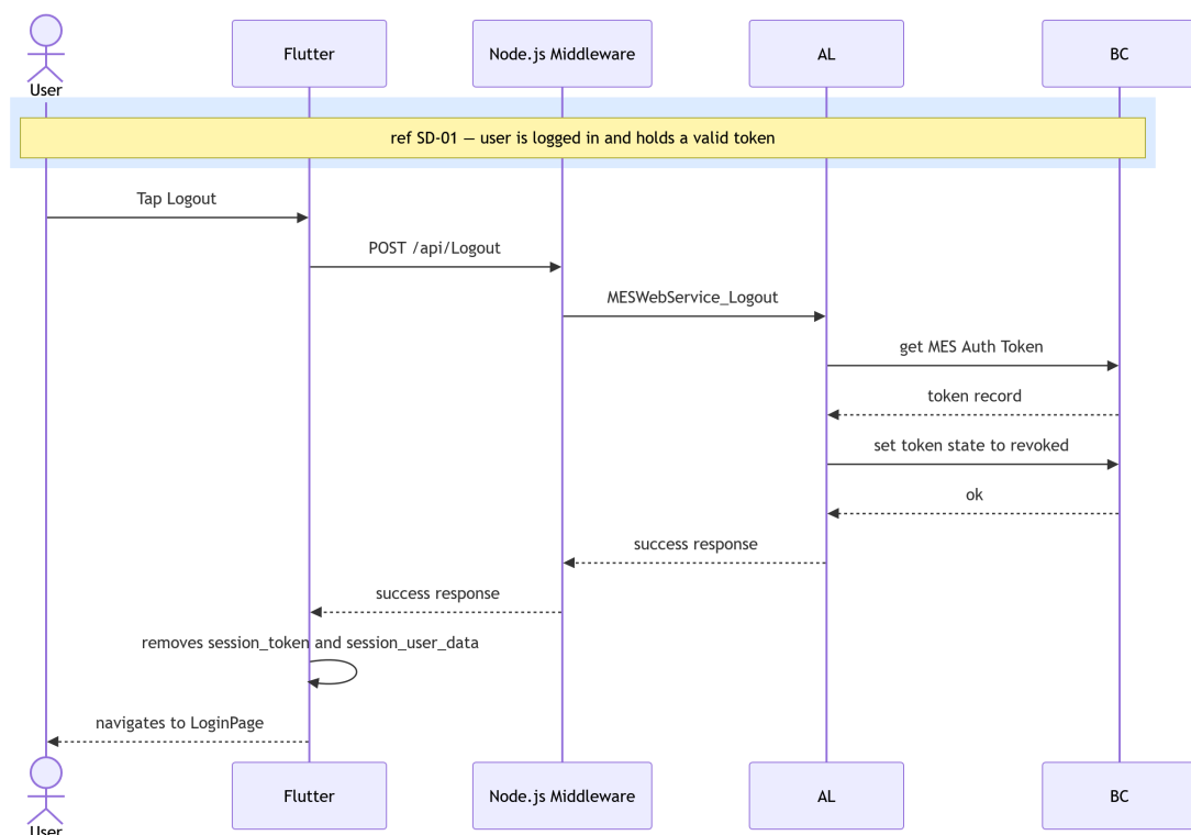
Figure 3.7. SD-03: Logout
