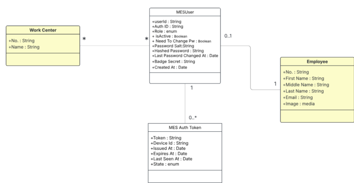
Figure 3.14. UML Class Diagram.
