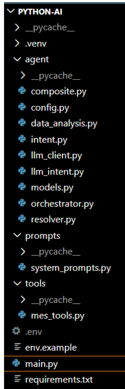
Figure 6.4. AI Assistant Layer
