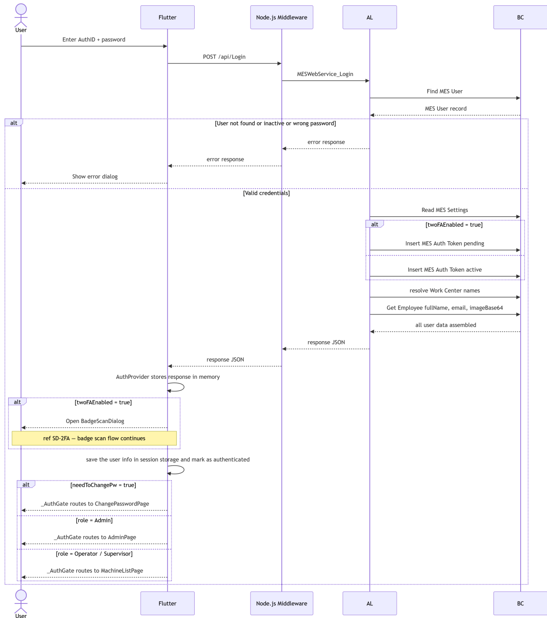
Figure 3.4. SD-01: Login.
