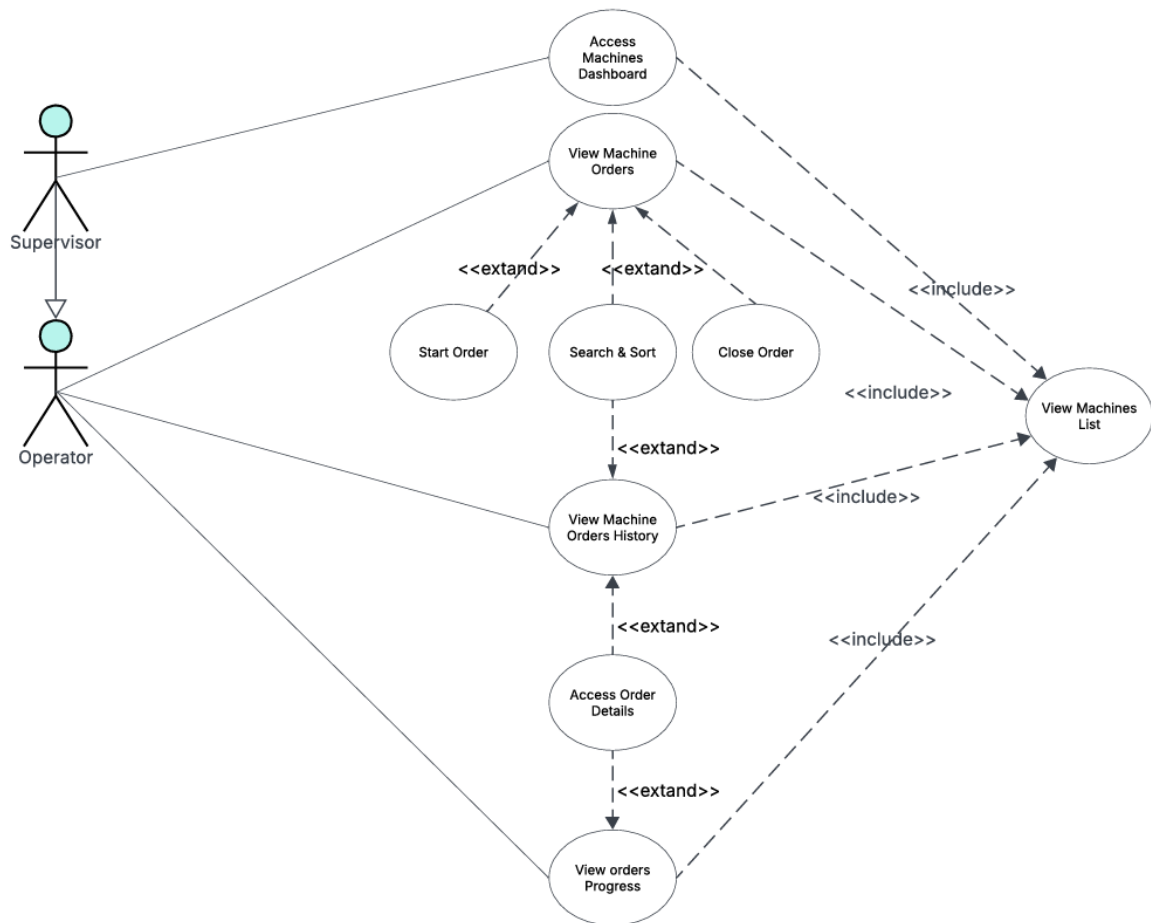
Figure 4.1. UML Use Case Diagram — Machine & Production Management.
