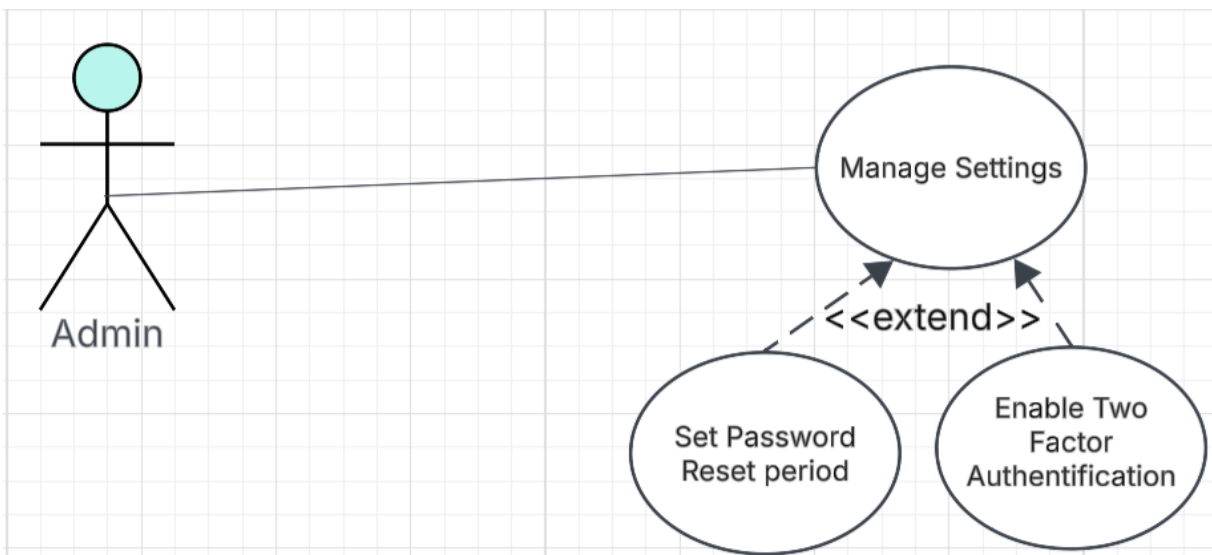
Figure 3.2. UML Use Case Diagram.
