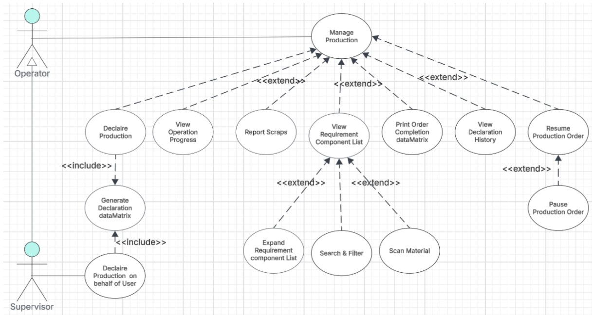
Figure 5.1. UML Use Case Diagram — Sprint 3
