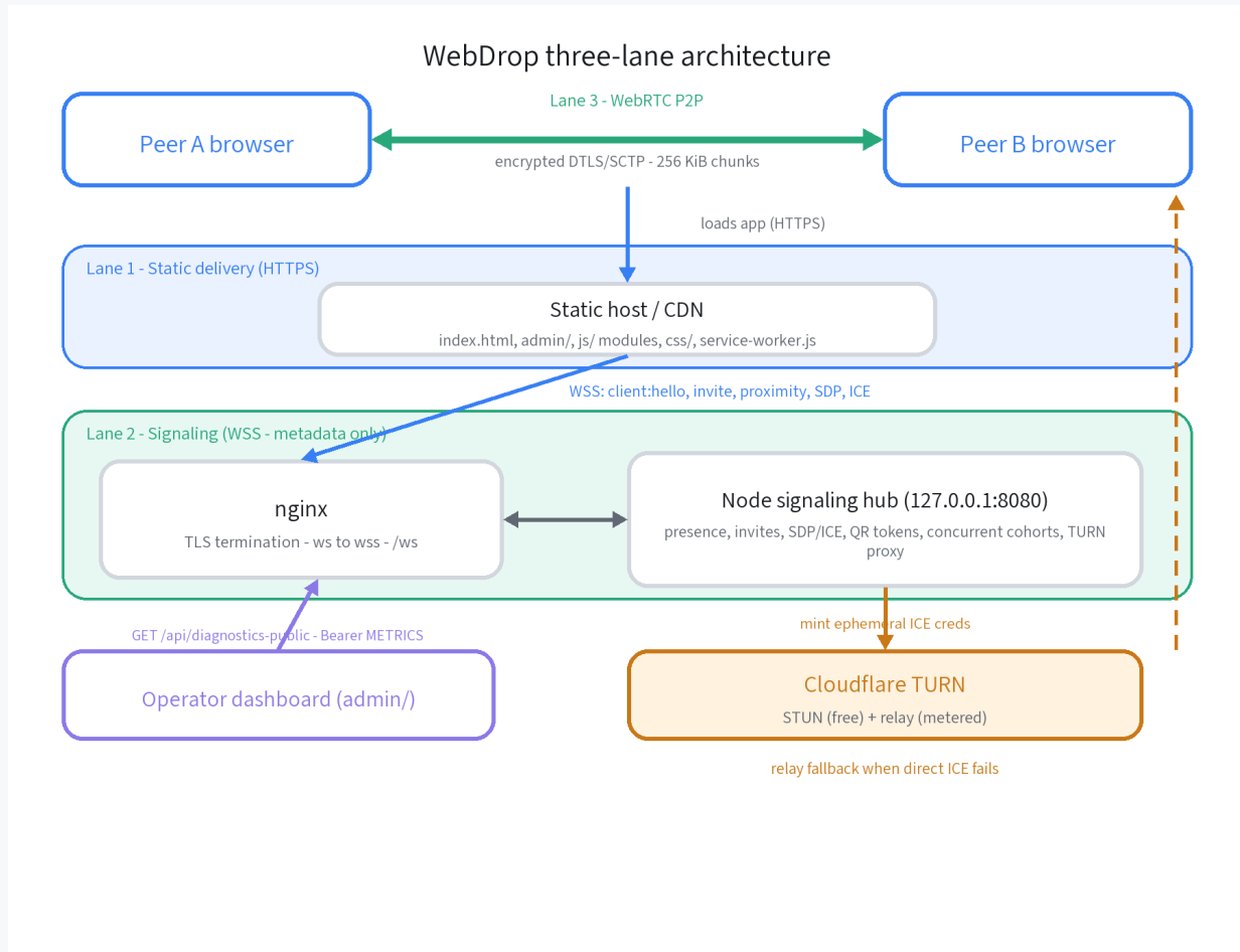
Figure 1 - WebDrop three-lane architecture
