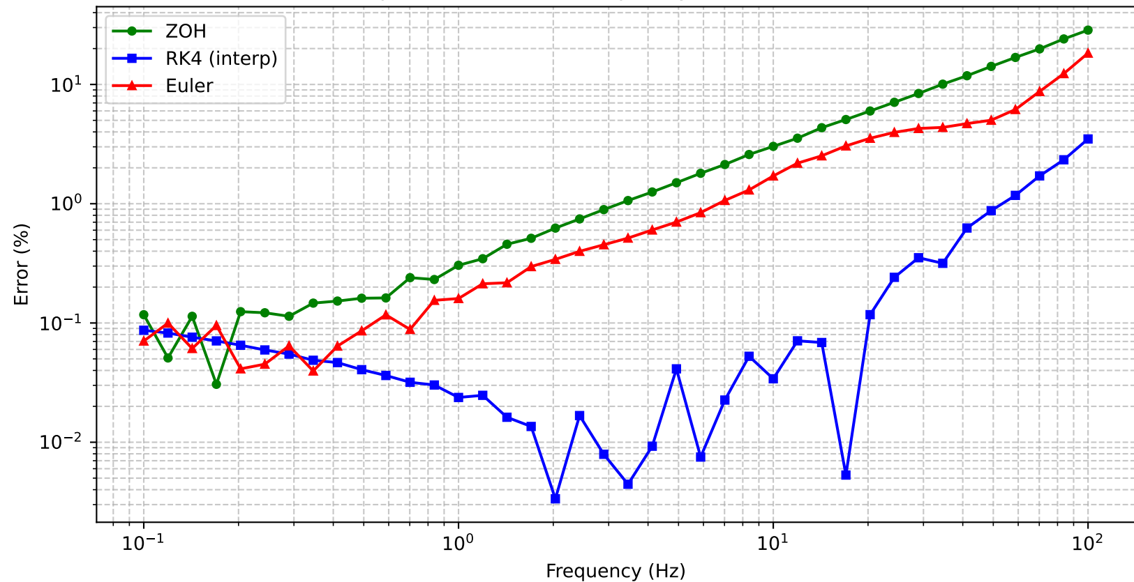
Impedance Error vs Frequency - Three Methods
