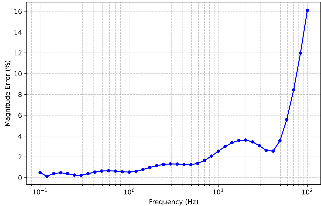
Approximation Error vs Frequency (n=5)
