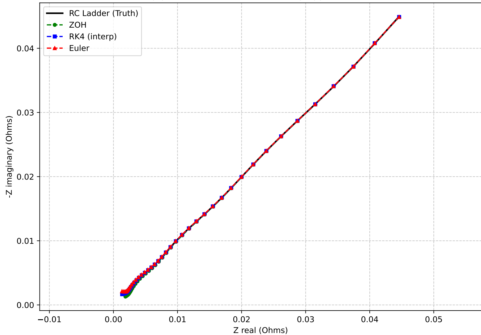
Nyquist Plot - RC Ladder Warburg Approximation
