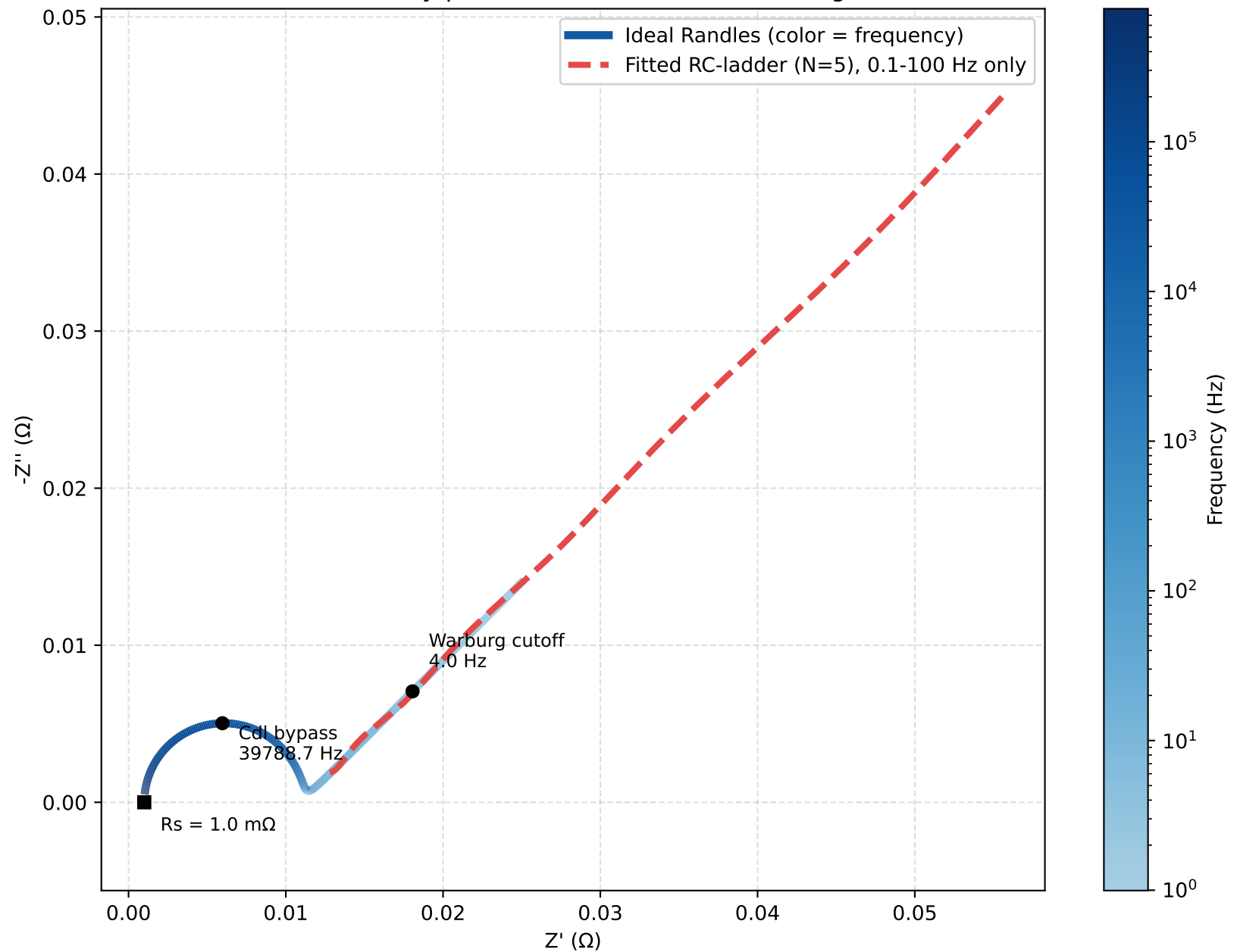
Randles Nyquist Plot: Ideal vs Fitted Warburg
