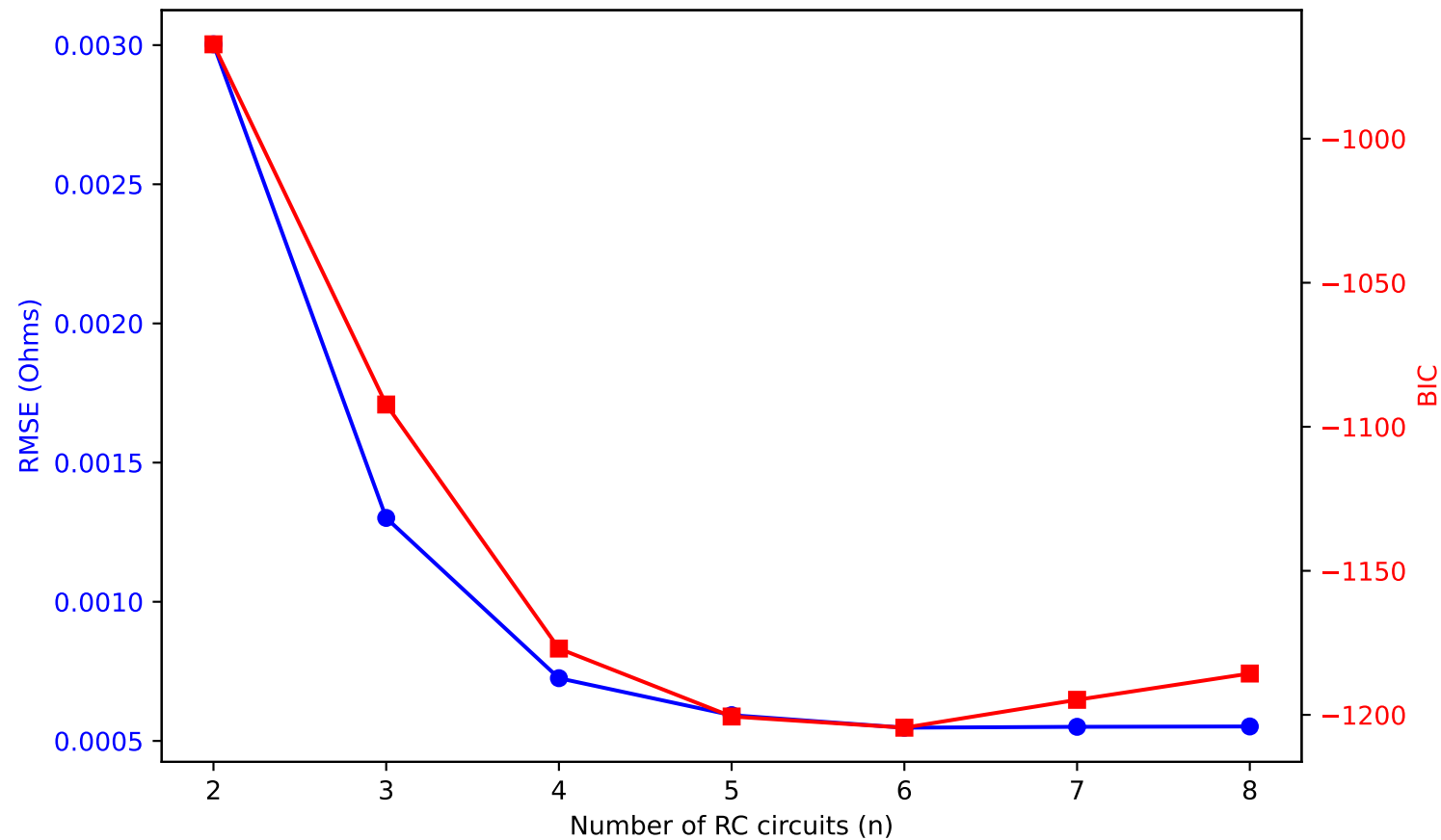
RMSE and BIC vs Number of RC Circuits (2% noise added)
