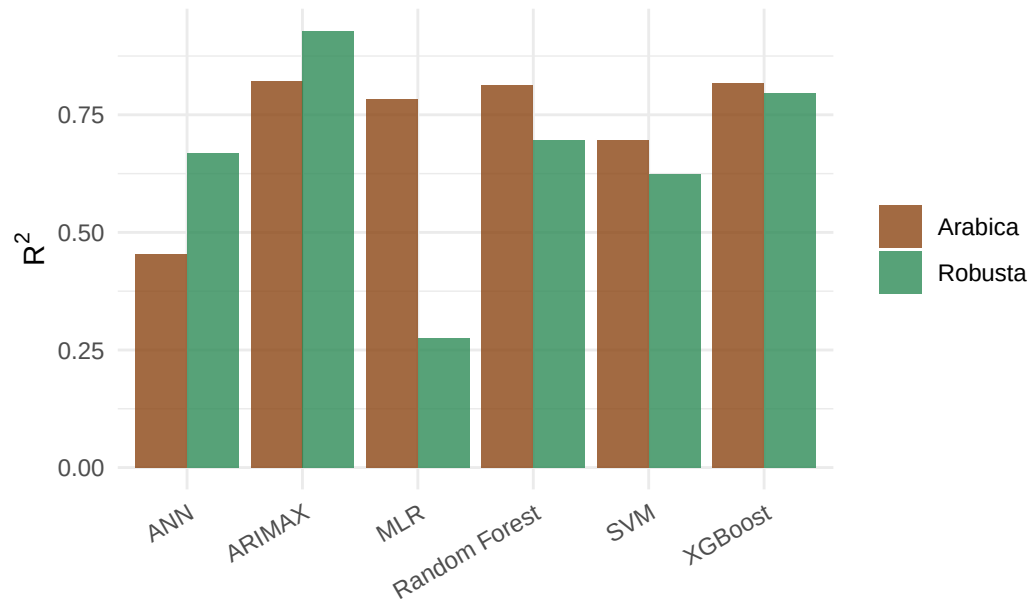
Out-of-sample R^2 by model and coffee variety
