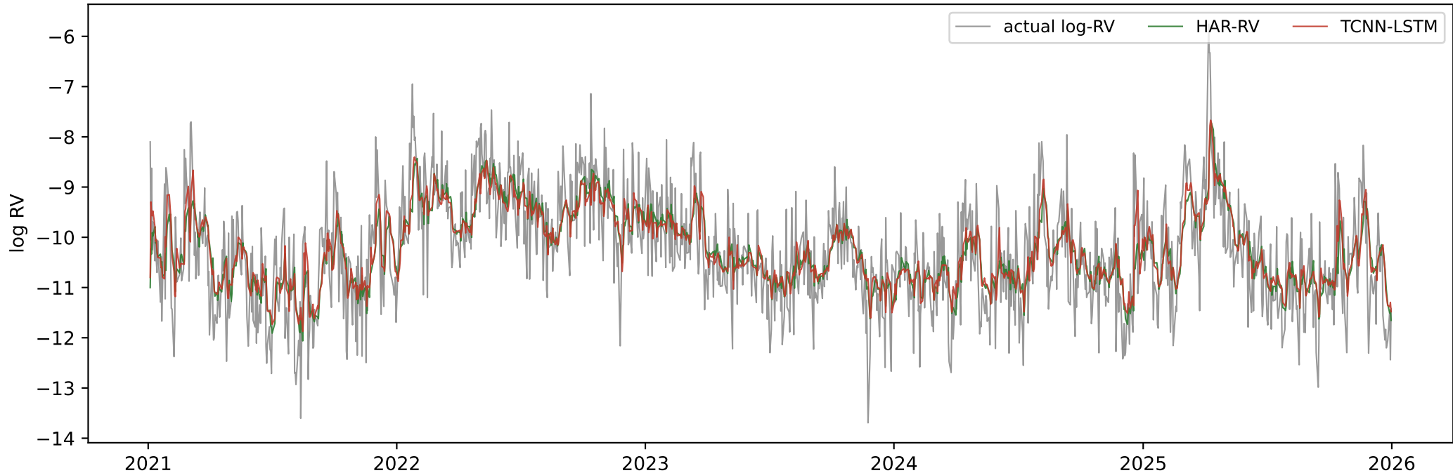
SPX test period: actual vs predicted log realized variance (2021-2026)
