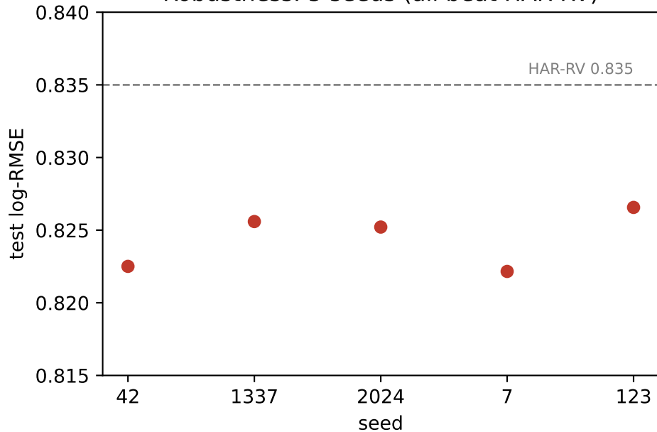
Robustness: 5 seeds (all beat HAR-RV)
