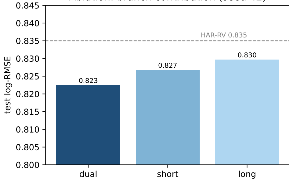
Ablation: branch contribution (seed 42)
