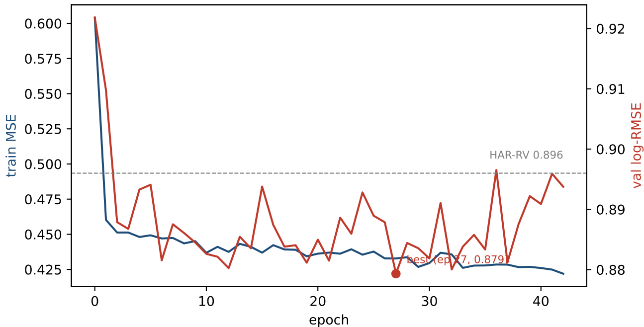
Dual-resolution TCNN-LSTM training (SPX, seed 42)
